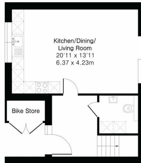
Ground Floor (Plot 07)
